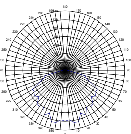
НСП-21ВEx-200-511
